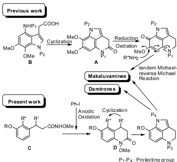
Scheme 1. Synthetic Strategies
