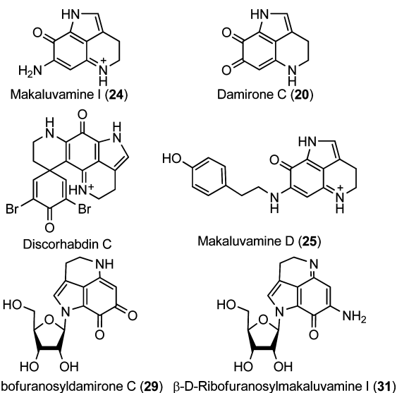
Figure 1. Tetrahydropyrroloiminoquinone alkaloids.
