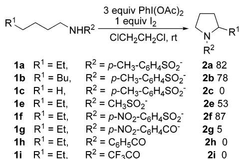
SCHEME 1. Intramolecular C–H Bond Amination of Amides
