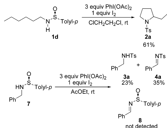
SCHEME 2. Oxidation of 4-Methylbenzenesulfonamides 1d and 7
