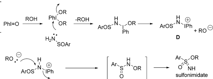
Scheme 4. Possible mechanism for the formation of sulfonylimides.
