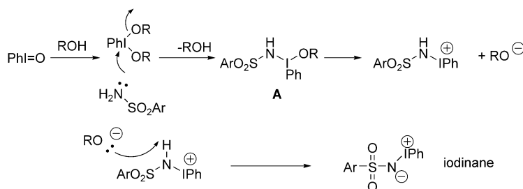
Scheme 2. Possible mechanism for the formation of phenyliodines.
