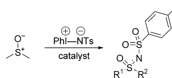
Scheme 1. General preparation of sulfoximines from sulfoxides.
