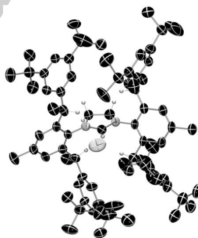
Figure 2. X-ray crystal structure of L8 ·HCl (the majority of the hydrogen atoms are omitted for clarity).
