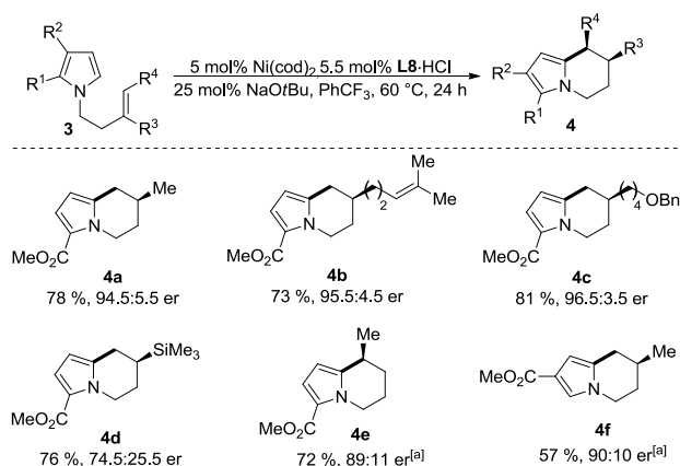
Scheme 3. Enantioselective C–H functionalization of pyrroles. Reaction conditions: 5 mol% Ni(cod) 2 , 5.5 mol% L8 -HCl, 25 mol% NaOtBu, 0.5 M in PhCF 3 at 60 °C for 24 h; [a] with 10 mol% Ni(cod) 2 , 11 mol% L8 -HCl, 50 mol% NaOtBu.
