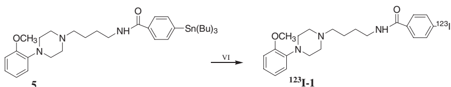
Scheme 2. [ ^{123}\text{I} ]-4-iodo- N -(4-(4-(2-methoxyphenyl)-piperazin-1-yl)butyl)-benzamide. (VI) [ ^{123}\text{I} ]-NaI, chloramine T, acetic acid, sodiummetabisulphite and ethanol
