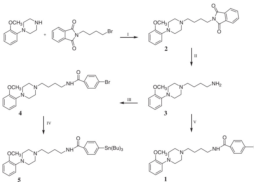
Scheme 1. Synthesis of N -(4-(4-(2-methoxyphenyl)-piperazin-1-yl)butyl)-4-tributylstannyl-benzamide and 4-iodo- N -(4-(4-(2-methoxyphenyl)-piperazin-1-yl)butyl)-benzamide. (I) Sodium carbonate and dimethylformamide, (II) hydrazine hydrate and ethanol, (III) 4-bromobenzoylchloride, triethylamine and dichloromethane, (IV) hexabutyliditin, tetrakis(triphenylphosphine)palladium and toluene, (V) 4-iodobenzoylchloride, triethylamine and dichloromethane
