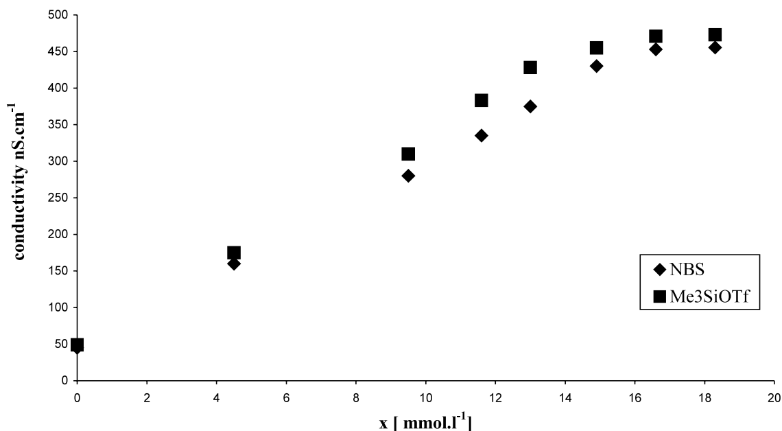
Fig. 2. The conductivity ( \chi ) as a function of the amount of electrophilic reagent added ( x ) to a solution of 0.53 \text{ mmol l}^{-1} of silane 1 in CHCl_3 .
