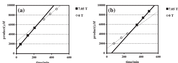
Figure 3. (a) The reaction course of the sample, 7.05 T \rightarrow 0 T. (b) The reaction course of the sample, 0 T \rightarrow 7.05 T.
