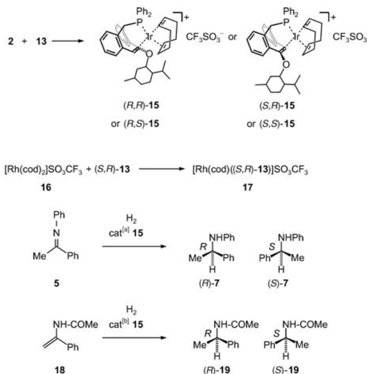
Scheme 5. Enantioselective catalytic imine hydrogenations with the iridium complexes ( R,R )- 15 , ( S,R )- 15 , ( S,S )- 15 , and ( R,S )- 15 . In the designation of the stereochemistry, the configuration at the benzylic carbon in the dibenzo[ a,d ]cycloheptene moiety is given first and the configuration at the ether carbon of the menthoxy group second. [a] s/c 100, p[\text{H}_2] = 50 bar, T = 50 °C. [b] s/c 50, p[\text{H}_2] = 50 bar, T = 50 °C.
