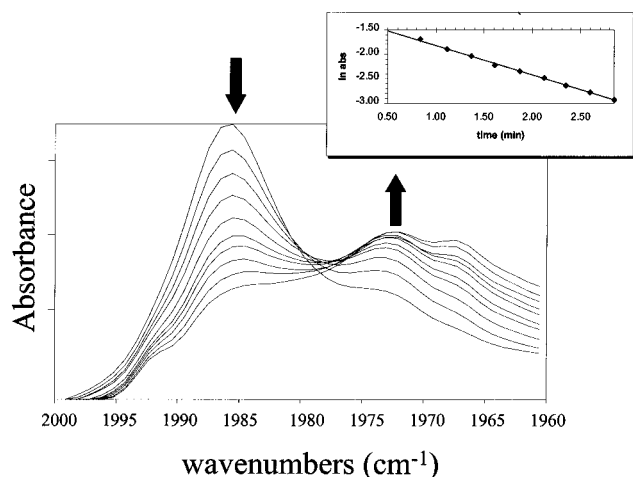
Figure 6. Spectral changes recorded for the process involving carbonyl ligand substitution in 2 with ^{13}\text{CO} at 30 °C. (Inset) Plot of \ln(\text{abs}) vs time (min) for this process, indicating first-order kinetics.
