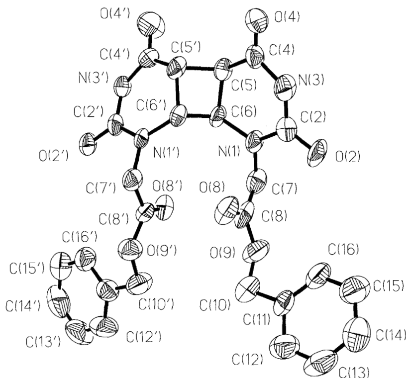
Fig. 3. ORTEP Plot of the molecular structure of compound 2 . Arbitrary numbering. Displacement ellipsoids are shown at the 50% probability level.
