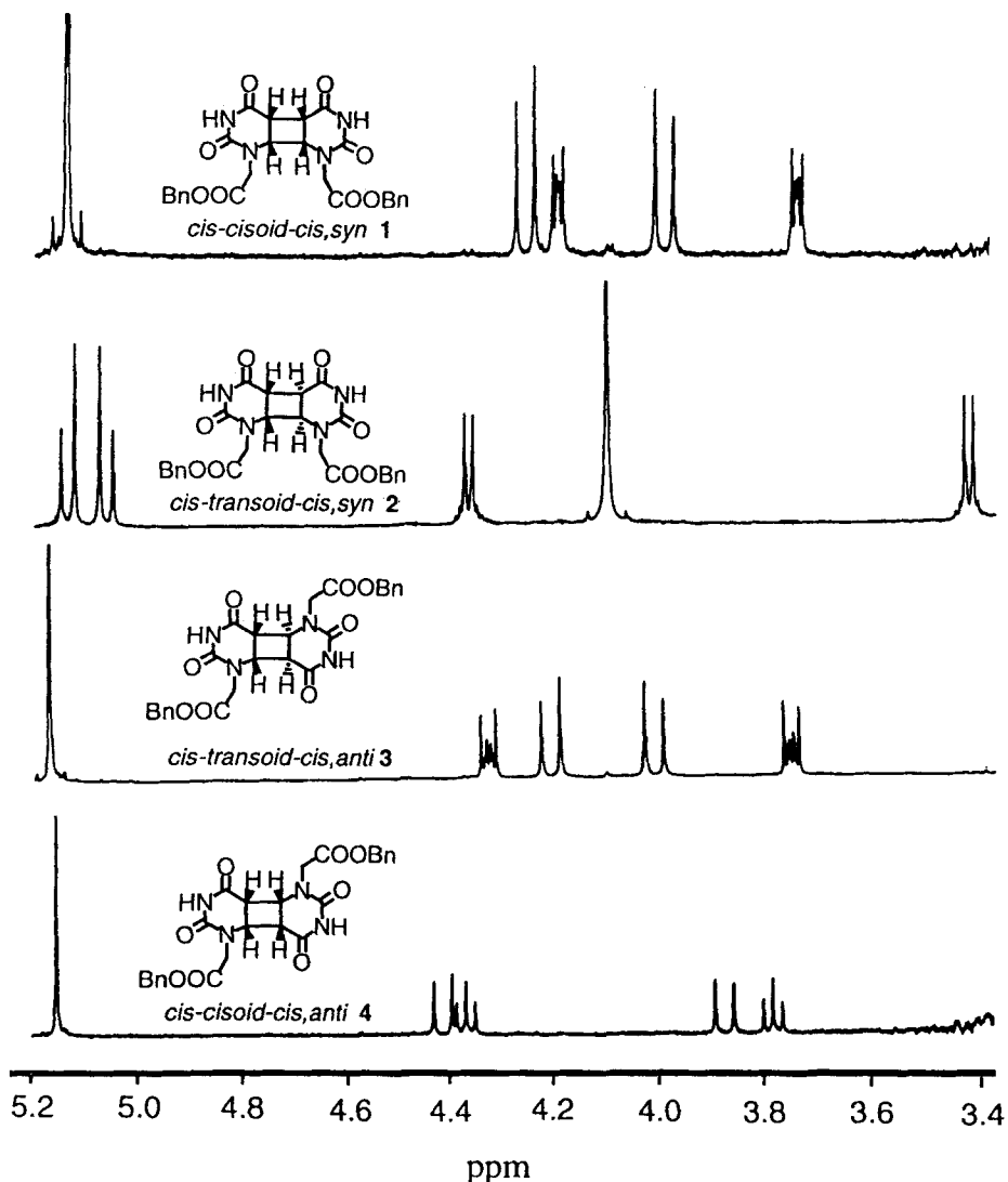
Fig. 5. 500-MHz 1 H-NMR Spectra ((D 6 )DMSO) of all four cyclobuta-fused uracil dimers 1–4
