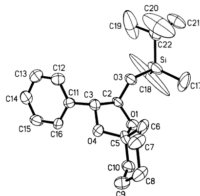
Fig. 1. The atomic arrangement in (2 R ,3 R )- 7 .
