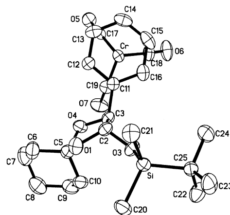
Fig. 2. The atomic arrangement in rac-trans -{[(1,2,3,4,5,6- \eta )-2- t -butyl(dimethyl)-(3-phenyl-1,4-dioxaspiro[4.5]decan-2-yl)oxy]silane}tricarboxylchromium ( 9/10 ).
