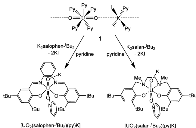
Scheme 1. Reaction of 1 with \text{K}_2(\text{salan-}^t\text{Bu}_2) and \text{K}_2(\text{salophen-}^t\text{Bu}_2)
