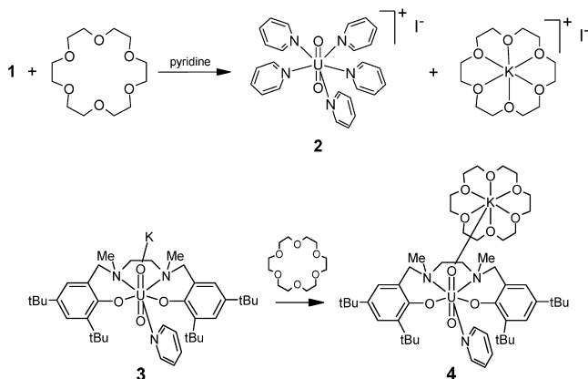
Scheme 2. Reaction of 1 and 3 with 18C6 Crown Ether in Pyridine
