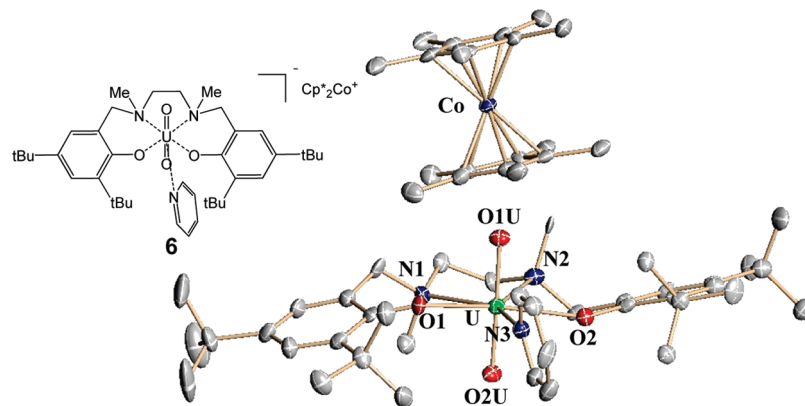
Figure 2. ORTEP view of 6 with thermal ellipsoids at the 30% probability level (hydrogen atoms were omitted for clarity) and schematic representation of the structure.
