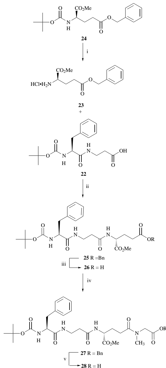
Scheme 5 Reagents, conditions (and yields): i, HCl, EtOAc, 0 °C (93%); ii, IBCF, NMM, THF, –30 °C → room temp. (95%); iii, H 2 , Pd/C, MeOH (91%); iv, IBCF, NMM, THF, –30 °C; then MeGlyOBn·pTsOH, NMM, THF, –30 °C → room temp. (80%); v, H 2 , Pd/C, MeOH (95%)
