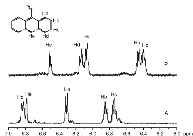
Figure 3. Partial 1 H NMR spectra of 1 in A) [D 8 ]THF and B) [D 8 ]THF/D 2 O (70:30 v/v).
