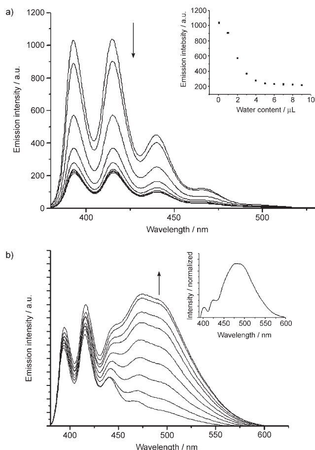
Figure 1. a) Water-driven fluorescence quenching of 1 ( c = 5 \times 10^{-6} M) in THF (3 mL); water was added in amounts of 0, 1, 2, 3, 4, 5, 6, 7, 8, and 9 \mu L, respectively. Inset: Plot of emission intensity versus quantity of added water in THF at 415 nm; \lambda_{\text{ex}} = 368 nm. b) Water-induced emission changes of 1 ( c = 5 \mu\text{M} ) in THF/H 2 O (from 9:1 to 3:1 v/v); \lambda_{\text{ex}} = 368 nm. Inset: Fluorescence differential spectrum of 1 from those in THF and H 2 O/THF (1:3 v/v).
