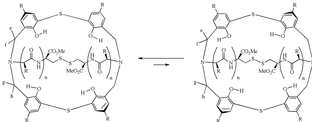
Figure 2. Schematic Representation of the Preferable Conformation of 1 .
