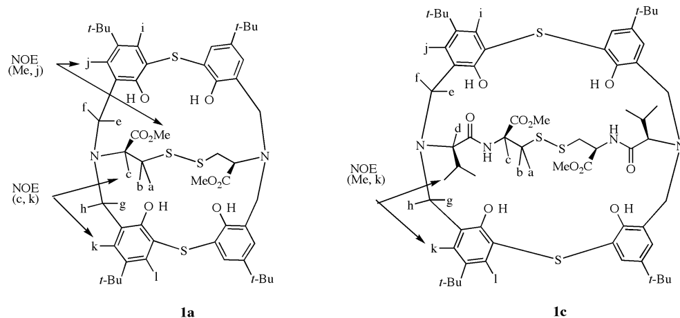
Figure 1. NOe Correlations.
