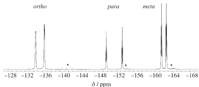
Figure 1. ^{19}\text{F} NMR spectrum of 7a (see text). Signals marked with asterisks belong to nonafluorobiphenyl derivatives [see 7' in Eq. (10)].
