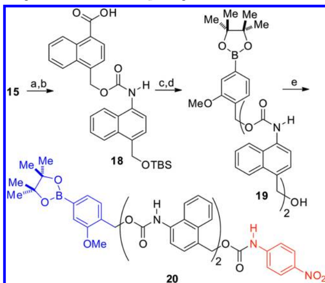
Scheme 4. Synthesis of Naphthalene-Based Carbamate Oligomer 20 with Two Repeating Units a
