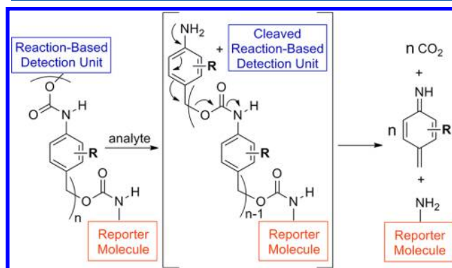
Figure 1. General mechanism of analyte-induced depolymerization in an aromatic poly(carbamate). Once the reaction-based detection unit is cleaved by reaction with a specific analyte, the repeating units of the polymer are released through successive azaquinone methide elimination reactions. Release of the reporter molecule is used to determine the kinetics of the depolymerization process.
