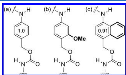
Figure 2. Three repeating units employed in the present study. The benzene-based repeating unit (a) serves as a reference point, while the m -methoxybenzene-based unit in (b) tests the effects of electron-donating groups on the rate of depolymerization. 18 The naphthalene-based unit in (c) tests the effects of aromaticity on the rate of depolymerization. Naphthalene is less aromatic than benzene as indicated by the relative aromaticity values of 0.91 and 1.0, respectively. 19
