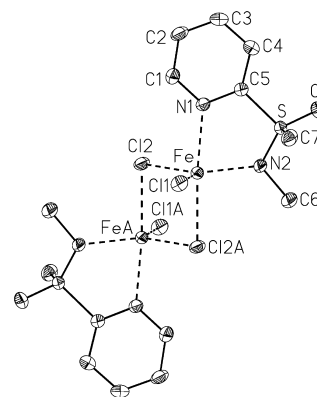
Figure 2. Structure of [\text{FeCl}_2\{\text{SO}(\text{NMe})\text{Me}(\text{NC}_5\text{H}_4)\}]_2 \cdot \text{THF} ( 6 ) without hydrogen atoms and THF solvent molecule (displacement ellipsoids are shown at the 50% probability level). Bond lengths (Å): Fe–Cl1 2.3033(9), Fe–Cl2 2.3915(8), Fe–Cl2A 2.4796(8), Fe–N1 2.204(3), Fe–N2 2.107(2), S–O 1.449(2), S–N2 1.551(3), S–C5 1.777(3), S–C7 1.770(3), N1–C1 1.338(4), N1–C5 1.341(4), N2–C6 1.491(4). Symmetry operation: A –x + 1, –y + 1, –z. Angles on S (deg): C5–S–C7 104.52(15), C7–S–O 107.66(16), C5–S–O 109.74(14), C5–S–N2 102.88(14), C7–S–N2 111.56(15), O–S–N2 119.43(15).
