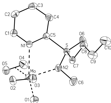
Figure 1. Structure of [\text{MoO}_2(\text{O}_2)_2\{\text{SO}(\text{NMe})^t\text{Bu}(\text{NC}_5\text{H}_4)\}] ( 5c ) without hydrogen atoms. (Displacement ellipsoids are shown at the 50% probability level.) Bond lengths (Å): Mo–O1 1.6869(13), Mo–O2 1.9353(13), Mo–O3 1.9645(13), Mo–O4 1.9554(13), Mo–O5 1.9255(13), Mo–N1 2.4038(14), Mo–N2 2.1750(14), S–O6 1.4498(12), S–N2 1.5746(15), S–C5 1.7854(17), S–C7 1.7917(17), N1–C1 1.335(2), N1–C5 1.344(2), N2–C6 1.497(2), O2–O3 1.4782(18), O4–O5 1.4804(19). Angles on S (deg): C5–S–C7 106.14(8), C5–S–O6 110.37(8), C7–S–O6 108.84(8), C5–S–N2 102.18(8), C7–S–N2 111.52(8), O6–S–N2 117.11(8).
