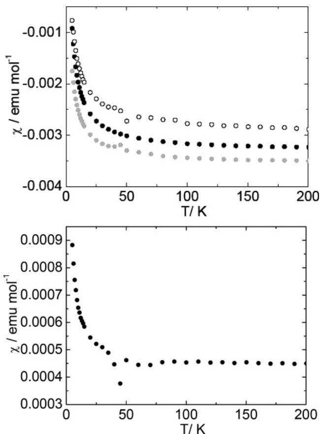
Figure 4. (a) Detail of the magnetic susceptibility of compound 2 (black circles), the thorium analogue (gray circles), and the sample holder (open circles), over the temperature range 5 – 200 K. The susceptibility of the sample holder has been scaled up by the same factor used to convert the measured to the molar susceptibility for 2 . (b) Residual molar susceptibility of 2 after correction for the diamagnetism of the sample and the sample holder.
