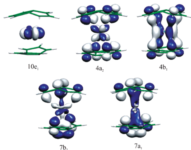
Figure 7. Frontier MOs of [Ce(C 8 H 6 ) 2 ]. The δ character of the ligand π frontier orbitals, with respect to the metal–ligand axis, closely resembles the e 2 orbitals of (C 8 H 8 ) 2− . 45
