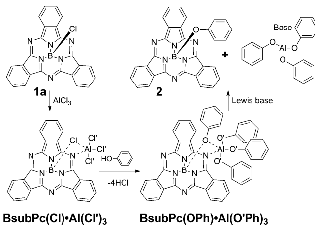
Scheme 1. Proposed Mechanism of Cl-BsubPc Activation to Reaction with Nucleophiles by Treatment with Aluminum Chloride
