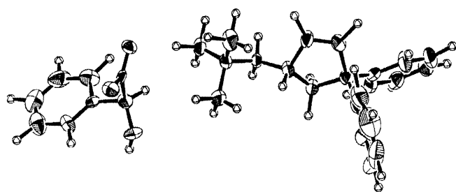
Fig. 3. ORTEP Drawing of the Crystal Structure of (-)-4·(S)-(+)-Mandelate Determined by X-Ray Crystallographic Analysis
