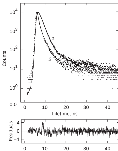
FIG. 5 Time-resolved fluorescence decay of polymer 4 ( \tau = 1.02 ns, \lambda_{\text{ex}} = 335 nm, \lambda_{\text{em}} = 390 nm, \chi^2 = 1.23 ) in tetrahydrofuran ( 1 ), the measured lamp pulse ( 2 ) and the weighted residuals
