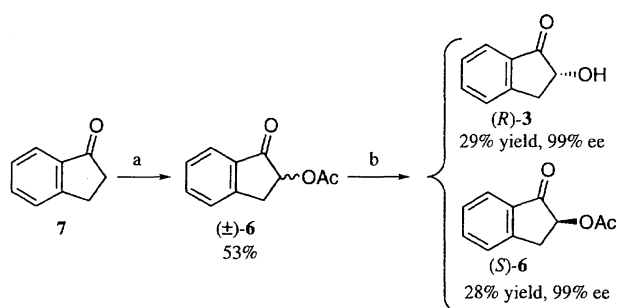
Scheme 4. Conditions: (a) Mn(OAc)_3 /benzene, (b) Pseudomonas sp. /phosphate buffer (pH 7)– CH_3CN .
