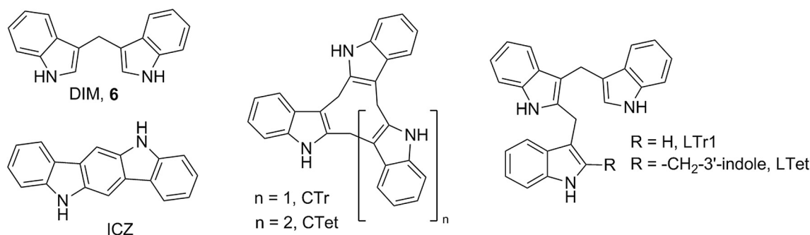
Fig. 2. The known metabolites/degradation products of indole-3-carbinol: 3,3'-diindolylmethane (DIM, 6 ), a cyclic tetramer (CTet), the first linear trimer (LTr1), indolo[3,2-b]carbazole (ICZ), a cyclic trimer (CTr) and a linear tetramer (LTet).
