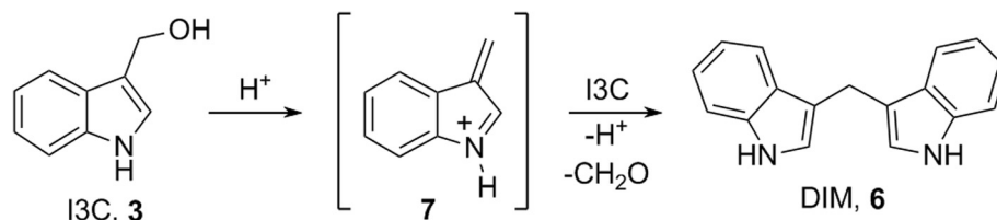
Scheme 1. The acid-catalysed conversion of I3C into DIM.
