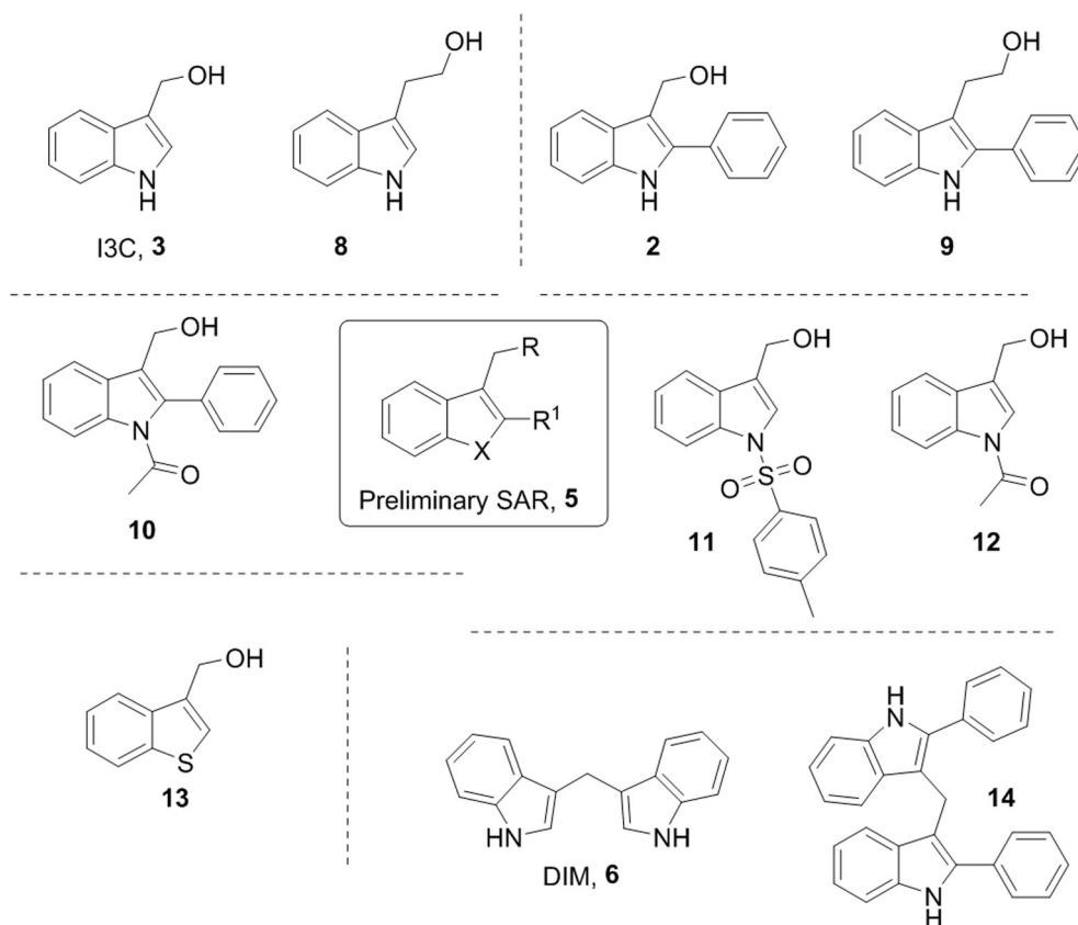
Fig. 3. SAR studied, grouped by feature being investigated.
