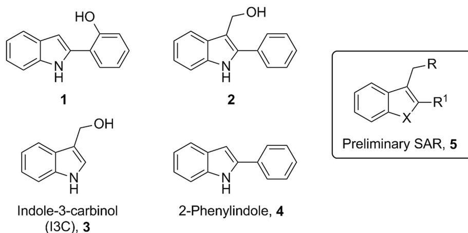
Fig. 1. The structures of 1–4 and the Markush structure ( 5 ) showing the preliminary SAR investigated. For R, R 1 and X – see Fig. 3.
