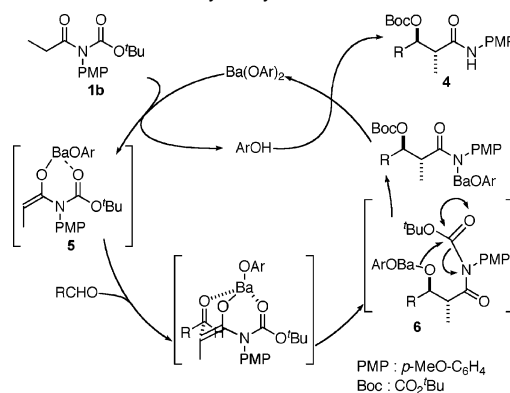
Scheme 1. Assumed Catalytic Cycle
