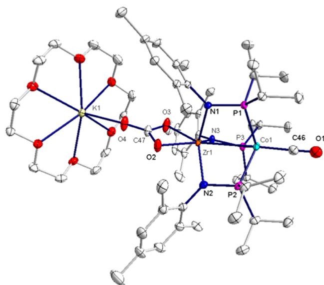
Figure 4. Displacement ellipsoid (50%) representations of [8][K(18-c-6)] . Hydrogen atoms were omitted for clarity. Relevant interatomic distances (Angstroms) and angles (degrees): Zr–Co, 2.8468(5); Zr–O2, 2.130(2); Zr–O3, 2.136(2); K–O4, 2.548(2); Co–C46, 1.750(4); O2–C47–O3, 110.6(3); K–O4–C47, 160.3(2); Co–C46–O1, 176.5(4).
