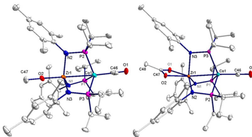
Figure 3. Displacement ellipsoid (50%) representations of 5 (left) and 7 (right). Hydrogen atoms were omitted for clarity. Relevant interatomic distances (Å) and angles (°). 5 : Zr–Co, 2.7499(14); Zr–O2, 1.912(5); Co–C46, 1.815(12); Co–Zr–O2, 174.43(16); Zr–O2–C47, 168.5(6); Co–C46–O1, 178.1(9). 7 : Zr–Co, 2.7110(5); Zr–O1, 2.244(2); Zr–O2, 2.253(2); Co–C46–O3, 178.8(3), O1–C47–O2, 117.7(3).
