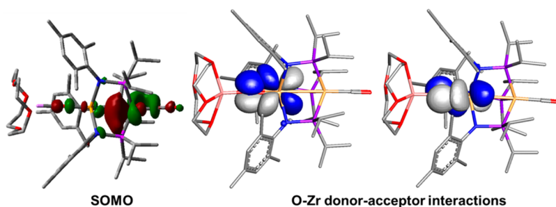
Figure 2. Calculated SOMO of [2][\text{Li}(\text{12-c-4})] (left) and \beta -orbital-derived O to Zr donor–acceptor interactions obtained via NBO calculations ( E_{\text{del}} = 16.3 and 14.7 kcal/mol, respectively). \alpha -Orbital-derived O to Zr donor–acceptor interactions are included in the Supporting Information (BP86/LANL2TZ(f)/6-311G(d)/D95 V).
