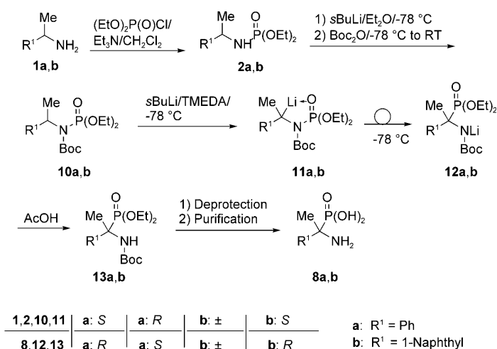
Scheme 3. Conversion of 1-phenyl- and 1-(1-naphthyl)ethylamines into quaternary \alpha -aminophosphonic acids 8a,b .
