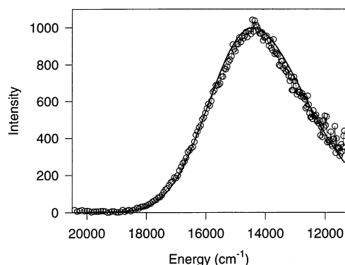
Figure 4. Normalized emission spectrum of fac -[(4,4'-Me 2 bpy)Re(CO) 3 (BIQD)] + in 1,2-dichloroethane at room temperature (O) and one-mode fit (—) with the parameters E_0 = 14\,920\text{ cm}^{-1} , S = 0.81 , \Delta\bar{\nu}_{1/2} = 2900\text{ cm}^{-1} and \hbar\omega = 1625\text{ cm}^{-1} .
