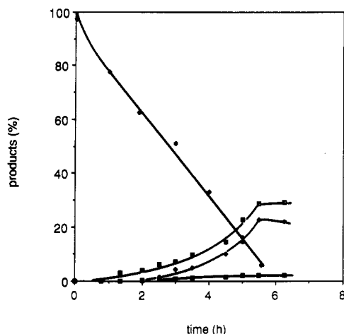
Figure 1. Reaction profile for the hydroxylation of phenol using [(\text{diphoe})\text{Pt}(\text{CF}_3)(\text{CH}_2\text{Cl}_2)]\text{BF}_4 as catalyst. Reaction conditions are as given in Table I. Products (%) is in reference to the \text{H}_2\text{O}_2 introduced. Symbols: ( \diamond ) \text{H}_2\text{O}_2 ; ( \blacklozenge ) hydroquinone; ( \square ) catechol; ( \blacksquare ) other products.
