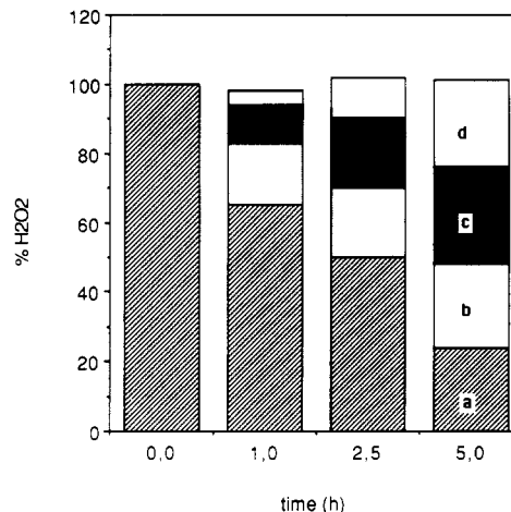
Figure 4. Mass balance at different reaction times of the hydrogen peroxide introduced in the hydroxylation of anisole using [(dppe)Pt(CF_3)(CH_2Cl_2)]ClO_4 as catalyst. Reaction conditions are as given in Table III. Symbols: (a) percent residual; (b) percent decomposed by the substrate; (c) percent decomposed by the catalyst; (d) percent converted into products.
