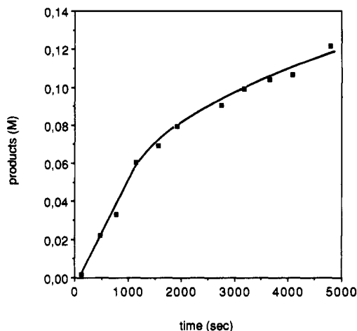
Figure 5. Typical reaction profile for total product formation in the hydroxylation of 1,3-dimethoxybenzene using [(diphoe)-Pt(CF 3 )(CH 2 Cl 2 )]BF 4 as catalyst, showing the linear initial rate. Reaction conditions: 1,3-dimethoxybenzene (neat), 60 mmol; 70% H 2 O 2 , 6 mmol; [Pt], 4.41 × 10 -3 M; T, 85 °C; N 2 , 1 atm.
