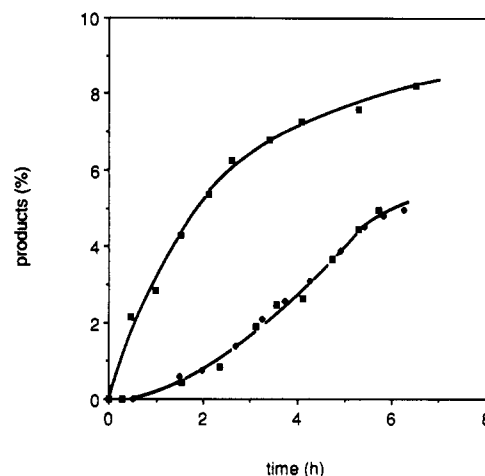
Figure 2. Comparison of the activity of [(\text{dppe})\text{Pt}(\text{CF}_3)(\text{CH}_2\text{Cl}_2)]\text{ClO}_4 ( \square ), (\text{dppe})\text{Pt}(\text{CF}_3)(\text{OH}) ( \blacklozenge ), and (\text{dppe})\text{Pt}(\text{CF}_3)(\text{OPh}) ( \blacksquare ) in the hydroxylation of phenol. Reaction conditions are as given in Table I. Products (%) is in reference to the \text{H}_2\text{O}_2 introduced.
