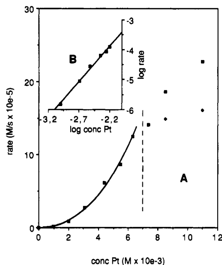
Figure 6. Effect of the concentration of [(diphoe)Pt(CF 3 )(CH 2 Cl 2 )]BF 4 on the initial rate in the catalytic hydroxylation of 1,3-dimethoxybenzene: (a) linear plot; (b) log/log plot. For concentrations higher than the broken line, the rate is controlled by the diffusion of H 2 O 2 from the aqueous to the organic phase. Diamonds represent experiments where the stirring rate was reduced to half. Reaction conditions: 1,3-dimethoxybenzene (neat), 60 mmol; 70% H 2 O 2 , 6 mmol; T, 85 °C; N 2 , 1 atm.
