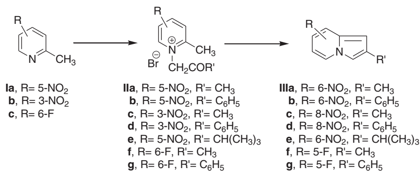
Scheme 1. Synthesis of indolizine derivatives IIIa–g .
