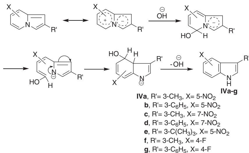
Scheme 2. Mechanism of formation of indole derivatives IVa–g .
