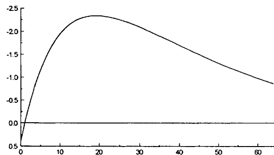
Figure 3. Optical rotation (degrees) as a function of time (h) for the rearrangement of 1-methylindene (1) catalysed by dihydroquinidine in o -dichlorobenzene at 20 °C
