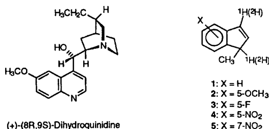
Figure 2. The amine catalyst (+)-(8 R ,9 S )-dihydroquinidine and the substrates 1-methylindene (1), 5-methoxy-1-methylindene (2), 5-fluoro-1-methylindene (3), 1-methyl-5-nitroindene (4) and 1-methyl-7-nitroindene (5)
