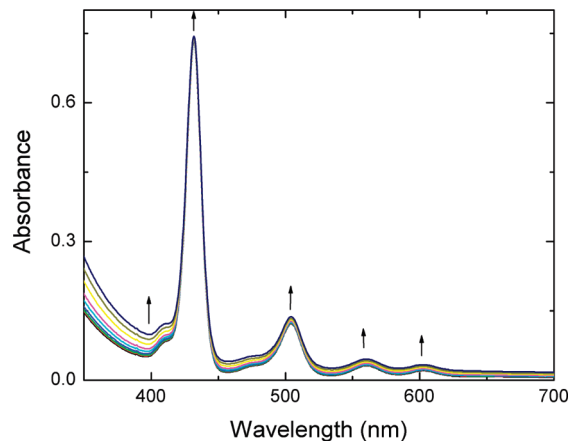
Figure 3. Absorption spectral changes observed during titration of BDP–zinc porphyrin–crown ether ( 3.6 \times 10^{-6} M) binding to C 60 ammonium cation ( 2.4 \times 10^{-4} M each addition) in benzonitrile.
