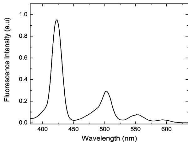
Figure 2. Excitation spectrum collected at 662 nm of the boron dipyrin–zinc porphyrin dyad in benzonitrile.
