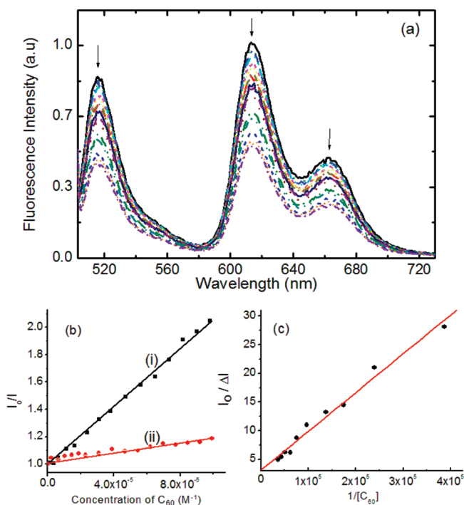
Figure 4. (a) Fluorescence spectral changes observed during increasing addition of C 60 ammonium cation (0.24 mM each addition) to a solution of BDP–zinc porphyrin–crown ether to form the triad in benzonitrile. \lambda_{\text{ex}} = 495 nm. (b) Stern–Volmer plots constructed for (i) C 60 ammonium cation and (ii) 2-phenyl fulleropyrrolidine quenching of BDP–zinc porphyrin–crown ether in benzonitrile (emission intensity of the 614 nm band of zinc porphyrin was monitored). (c) Benesi–Hildebrand plot constructed by monitoring the emission intensity at 614 nm band for calculating the binding constant. The abbreviations I_0 and I represent fluorescence intensity in the absence and presence of fullerene, and \Delta I is the change of fluorescence intensity upon addition of fullerene.
