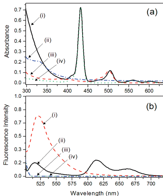
Figure 1. (a) UV–visible spectra of (i) BDP–zinc porphyrin–crown ether dyad (0.32 \mu M), (ii) C 60 ammonium cation (0.12 mM), (iii) p -tolyl boron dipyrin (BDP control, 0.32 \mu M), and (iv) zinc porphyrin–crown ether (0.32 \mu M) in benzonitrile. (b) Fluorescence spectra of (i) BDP control (0.32 mM), (ii) BDP–zinc porphyrin–crown ether dyad (0.32 \mu M), (iii) zinc porphyrin–crown ether control (0.32 \mu M), and (iv) C 60 ammonium cation (0.12 mM) in benzonitrile. The compounds were excited at \lambda_{\text{ex}} = 495 nm.
