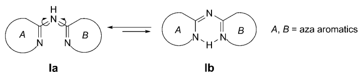
Scheme. Tautomers 1a and 1b in Neutral Solution
