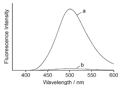
Figure 10. Fluorescence spectra of an aqueous solution of 4 ( [4] = 0.24 mM) (a) and a resolubilized aqueous solution of SWNTs/ 4 (b) (concentration of 4 was estimated to be 0.24 mM). Excitation wavelengths for (a) and (b) are 367 and 357 nm, respectively.
