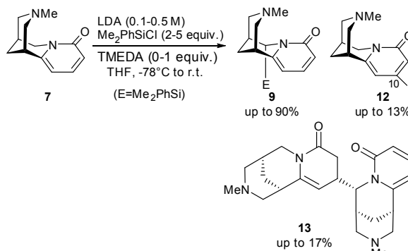
Scheme 3. Optimization of C(6) lithiation. Variables evaluated were substrate concentration, equivalents of LDA and Me 2 PhSiCl, and presence of TMEDA (key to a high yield of 9 ) Details are available in the Supplementary Information.
