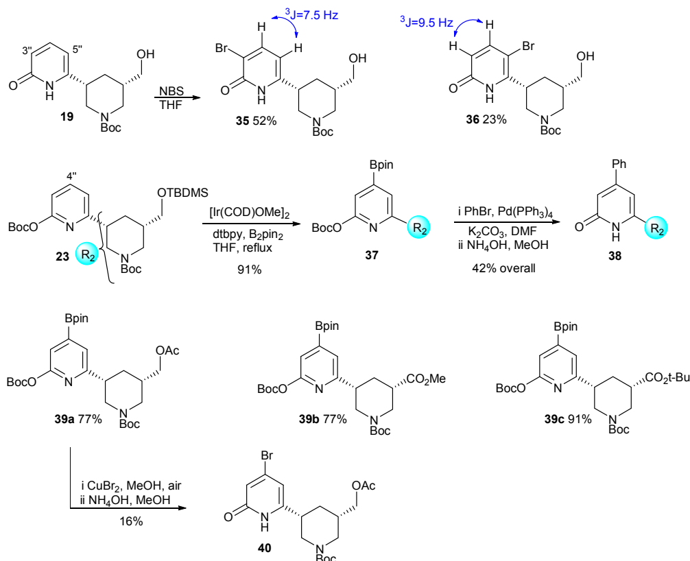
Scheme 11. Pyridone functionalisation.
