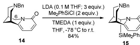
Scheme 4. C(6) Lithiation and silylation of N-benzylcytosine 14 .
