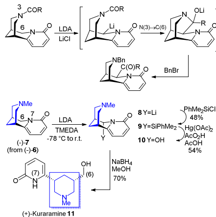
Scheme 2. Top: C(6) Lithiation triggering N(3)→C(6) acyl migration (Rouden et al 13 ). Bottom: C(6) Oxidative functionalisation of N-methylcytisine 7 ; a biomimetic synthesis of (+)-kuraramine 11 (Gallagher et al 14 ).
