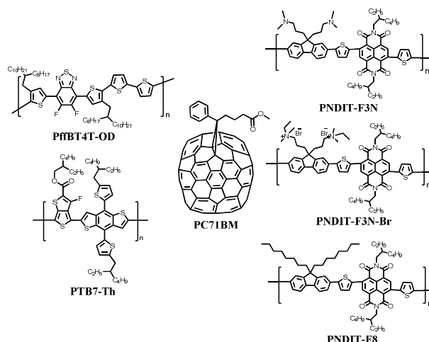
Chart 1. Chemical structures of PffBT4T-OD, PTB7-Th, PNDIT-F3N, PNDIT-F3N-Br, PNDIT-F8 and PC 71 BM.
