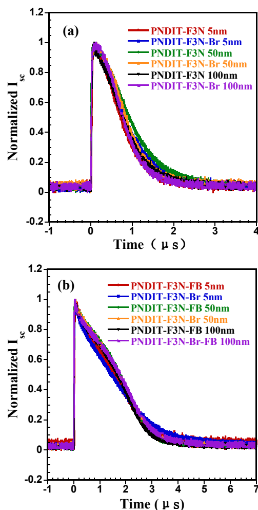
Figure 6. Transient photocurrent of different BHJ systems PTB7-Th:PC 71 BM (a) and PffBT4T-OD/PC 71 BM (b) based PSC devices with different ETLs.
