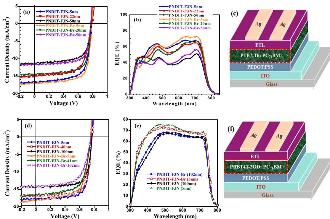
Figure 2. (a) J-V curves of PSC devices using PTB7-Th:PC 71 BM as the active layer with different ETLs in various thickness. (b) EQE of the devices using PTB7-Th:PC 71 BM as the active layer with different ETLs in various thickness. (c) Device structure of the PTB7-Th:PC 71 BM BHJ based PSCs. (d) J-V curves of PSC devices using PffBT4T-2OD: PC 71 BM as the active layer with different ETLs in various thickness. (e) EQE of the devices using PffBT4T-2OD: PC 71 BM as the active layer with different ETLs in various thickness. (f) Device structure of the PffBT4T-2OD: PC 71 BM BHJ based PSCs.
