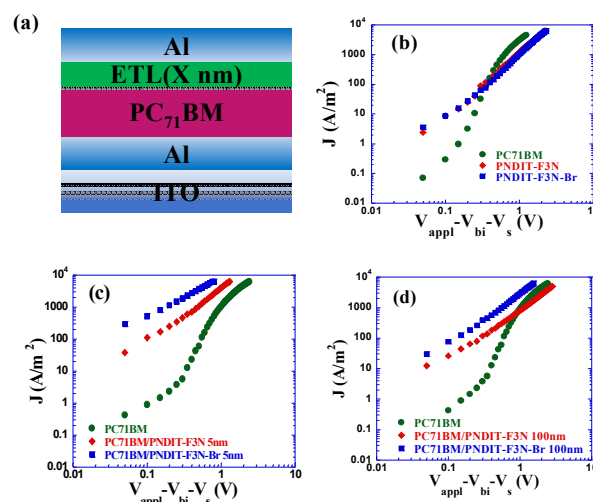
Figure 3. The structure of electron only devices (a).and J-V curves of electron only devices.
