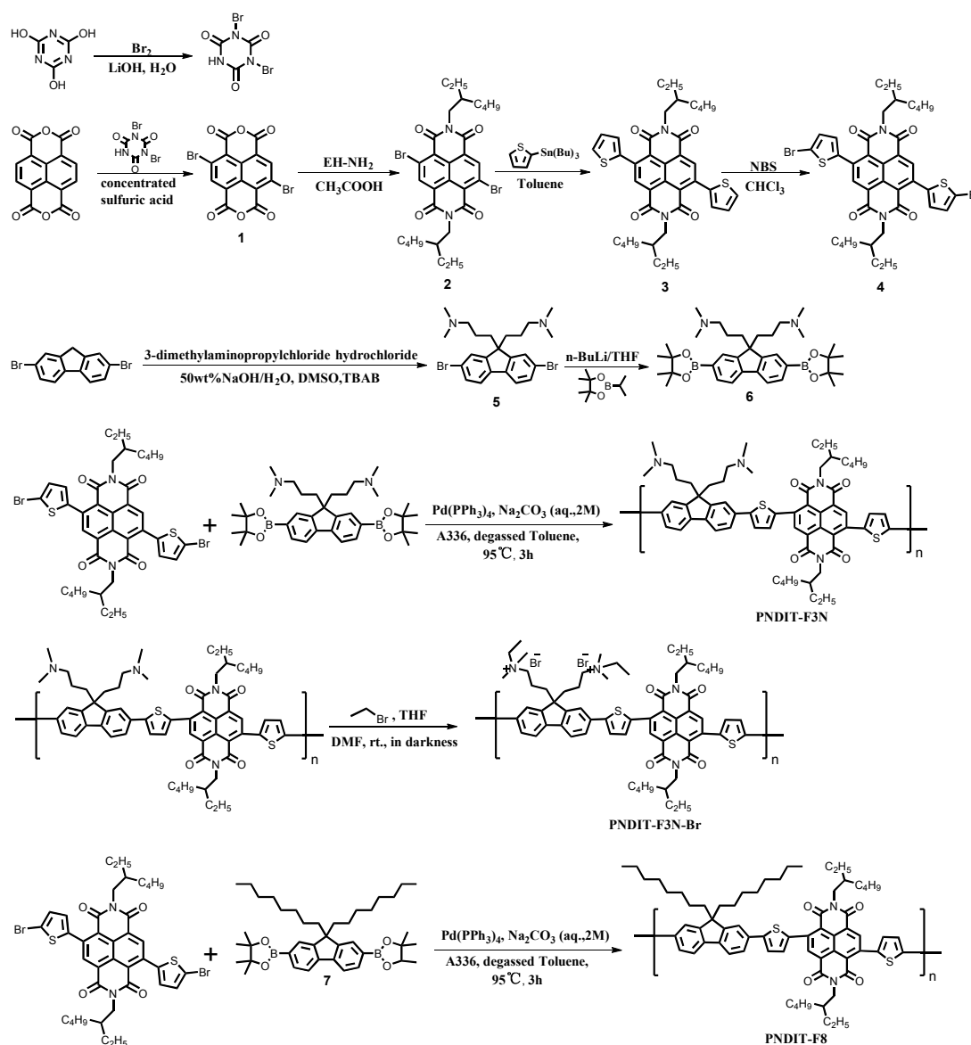
Scheme 1. Synthesis of n-type WSCPs PNDIT-F 3 N, PNDIT-F 3 N-Br and n-type semiconducting polymer PNDIT-F8.
