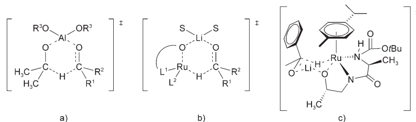
Figure 3. a) Cyclic transition state for the aluminium alkoxide mediated reduction of ketones by 2-propanol (Meerwein–Pondorff–Verley reduction). b) Proposed schematic cyclic transition state involved in the \text{Ru}^{\text{II}} -(arene)–pseudo-dipeptide-catalyzed reduction of ketones in the presence of lithium salts. c) Possible geometry of the transition state showing the important interactions between the ruthenium hydride, the lithium cation, and the substrate.
