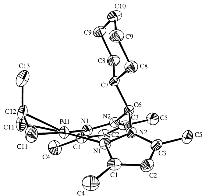
Fig. 4. ORTEP view with atomic numbering of the cation of 5 (30% probability ellipsoids). Proton atoms have been omitted for clarity.
