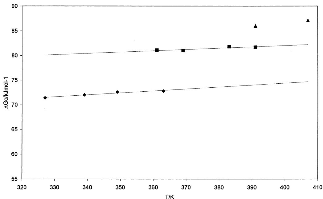
Fig. 2. Linear plot of \Delta G^\ddagger ( \text{kJ mol}^{-1} ) vs. T_c for the isomerization process of complex 4 in 1,1',2,2'-tetrachloroethane- d_2 : (■) 1.6 \times 10^{-2} \text{ mol l}^{-1} (▲) 0.8 \times 10^{-2} \text{ mol l}^{-1} (◆) Addition of 5.14 mg of \text{PPh}_4\text{Cl} ( 1.37 \times 10^{-2} \text{ mmol} ) to 0.50 ml of the 1.6 \times 10^{-2} \text{ mol l}^{-1} solution of complex 4 .
