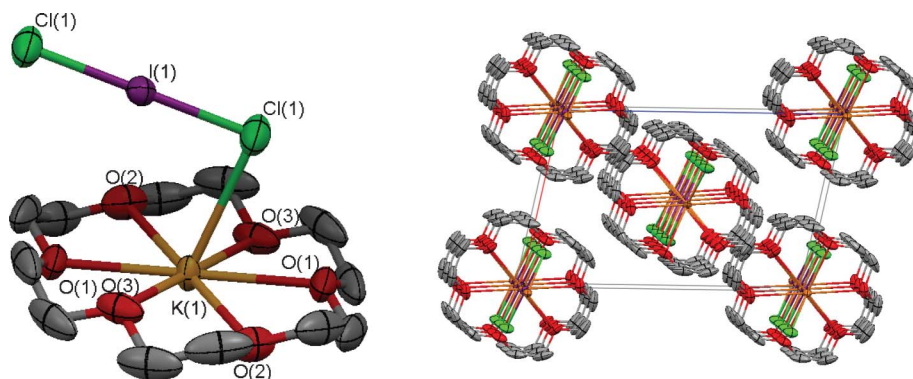
Fig. 1 ORTEP diagram of \text{[K·18-Crown-6]ICl}_2\text{]} complex showing 50% thermal ellipsoids. Hydrogen atoms are omitted for clarity (left). Packing of coordination polymer of \text{[K·18-C-6]}^+ cations and bridging \text{ICl}_2^- anions (right).
