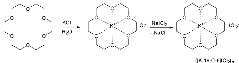
Scheme 1 Synthesis of \text{[K·18-C-6]ICl}_2\text{]}_n .
