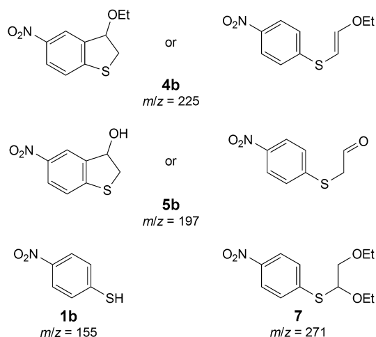
Fig. 6. Structures of the intermediates in the synthesis of 5-nitrobenzothiophene.
