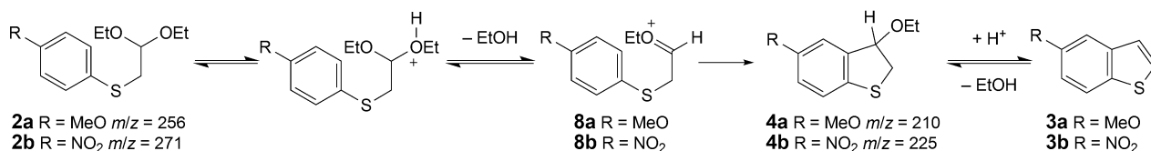
Scheme 3. Proposed reaction mechanism.
