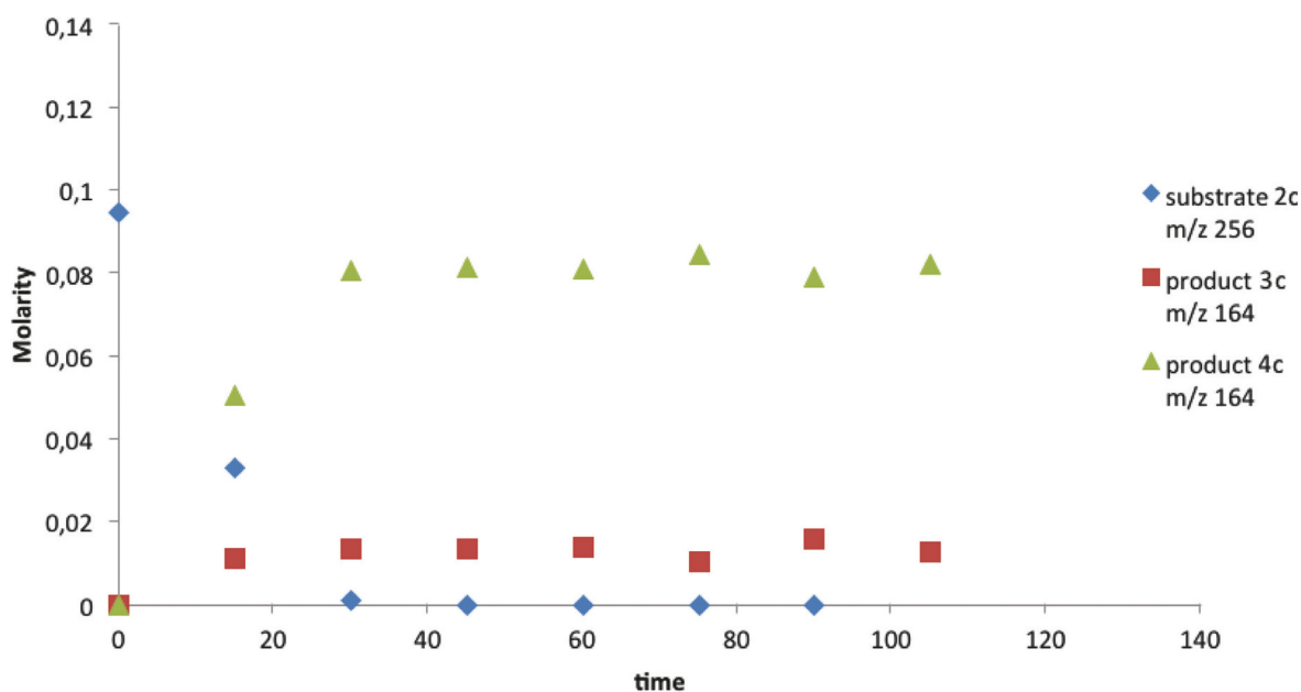
Fig. 7. Kinetics of the reaction 2c \rightarrow 3c + 4c .
