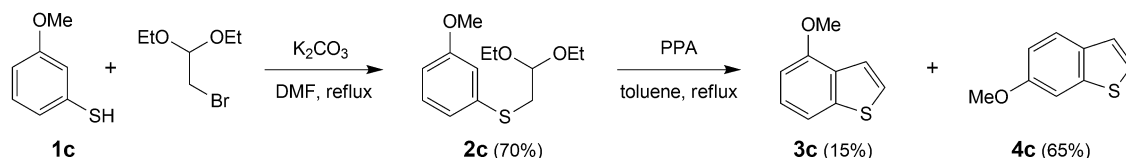
Scheme 2. Synthesis of 3c and 4c .
