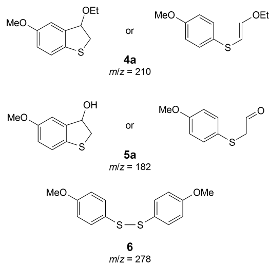
Fig. 3. Structures of intermediates and disulfide in the synthesis of 5-methoxybenzothiophene.
