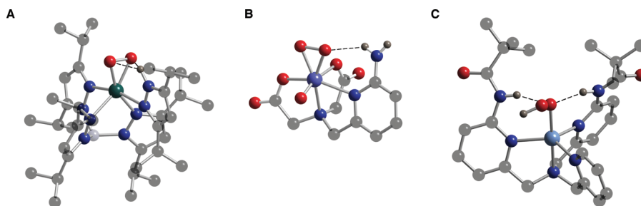
Figure 10. Molecular structures of metal–peroxo complexes with intramolecular H bonds: [\text{Mn}^{\text{III}}(\text{O}_2)] (A); 33 [\text{V}^{\text{V}}(\text{O}_2)(\text{O})]^- (B); 34 [\text{Cu}^{\text{II}}(\text{OOH})]^+ (C). 35c
