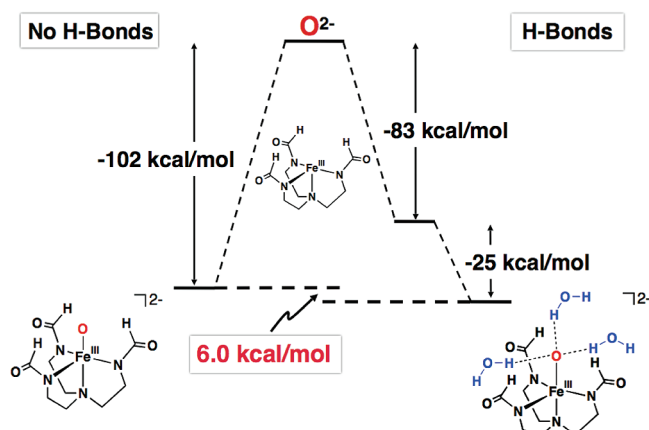
Figure 17. Bonding decomposition scheme for the Fe^{III}-O complex illustrating the effects of the intramolecular H-bonding network.
