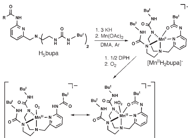
Figure 10. Molecular structures of metal–peroxo complexes with intramolecular H bonds: [\text{Mn}^{\text{III}}(\text{O}_2)] (A); 33 [\text{V}^{\text{V}}(\text{O}_2)(\text{O})]^- (B); 34 [\text{Cu}^{\text{II}}(\text{OOH})]^+ (C). 35c
