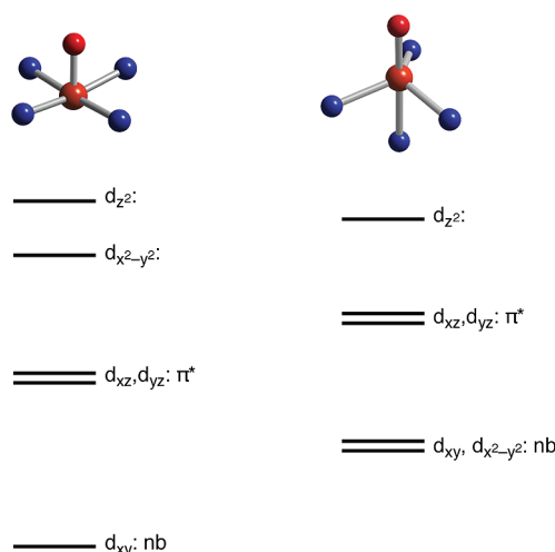
Figure 16. Qualitative orbital diagrams for metal–oxo complexes with C_{4v} (left) and C_3 symmetry (right) (adapted from Mayer and Thorn). 48
