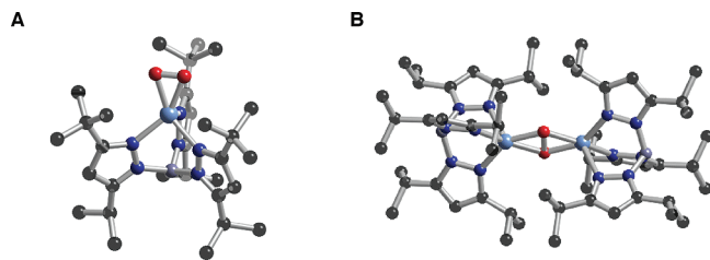
Figure 6. Molecular structures of copper-superoxo complex [CuTp t -Bu 2 Pr-(η 2 -O 2 )] (A) and μ-η 2 :η 2 -peroxodicopper(II) complex [Cu II Tp t Pr 2 Pr] 2 (O 2 ) (B) showing the controlling effects of steric bulk.
