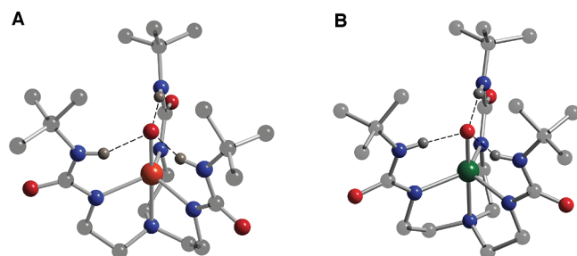
Figure 15. Molecular structures of [Fe^{III}H_3buea(O)]^{2-} (A) and [Mn^{III}H_3buea(O)]^{2-} (B) determined by XRD methods.
