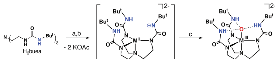
Scheme 3. Synthetic Procedure for the Isolation of [M^{III}H_3buea(O)]^{2-} ( M^{III} = Fe, Mn ) a
