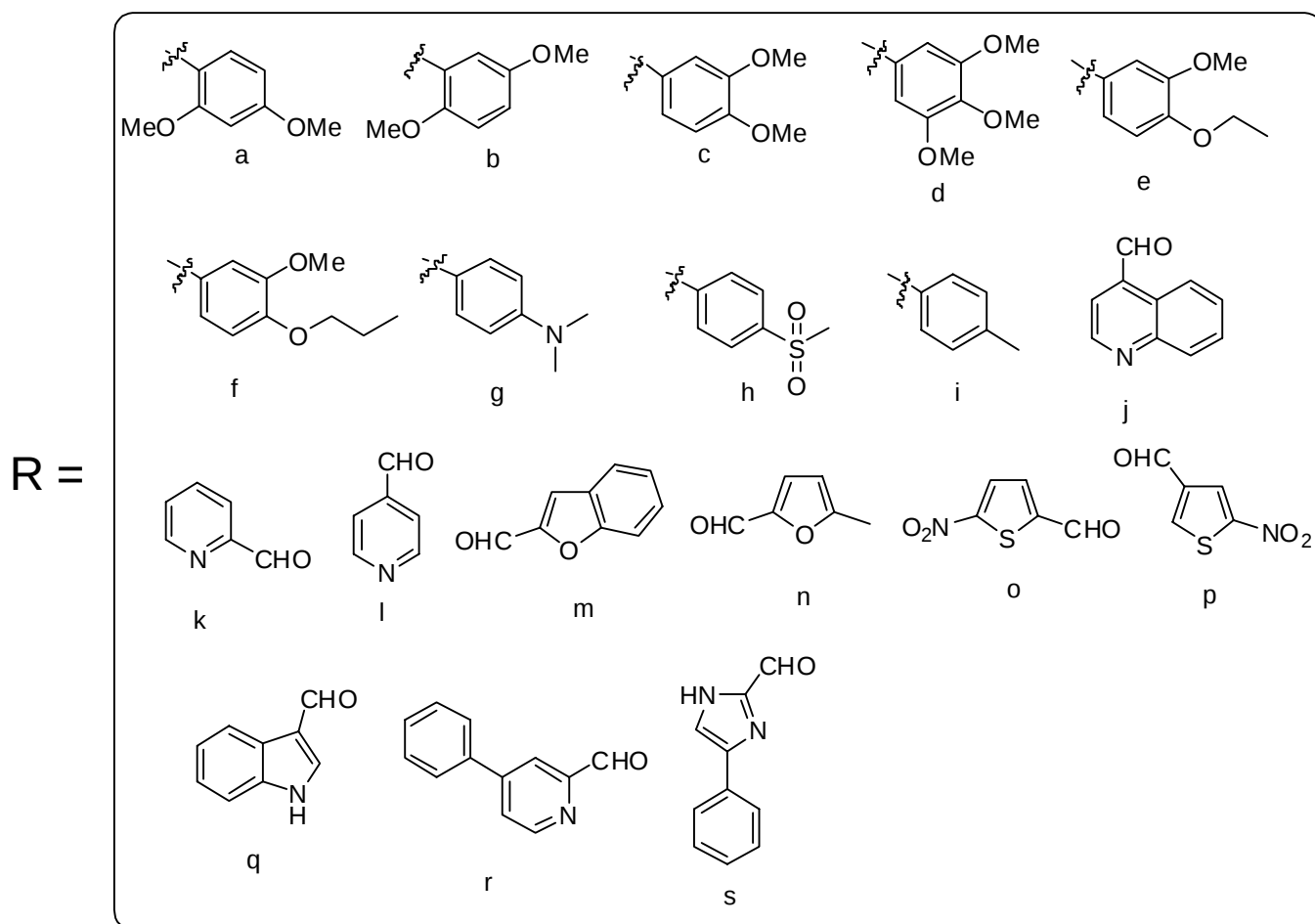
Scheme-1: Synthesis of hydrazone derivatives of 4-(4-chlorophenyl)cyclohexane carboxylic acid ( 4a-s ); Experimental conditions: (a) Conc; \text{H}_2\text{SO}_4 , methanol, reflux, 10 h; (b) \text{NH}_2\text{NH}_2 \cdot \text{H}_2\text{O} , ethanol, reflux, 3 h; (c) Benzaldehydes ( a-s ), ethanol, reflux, 1 h
