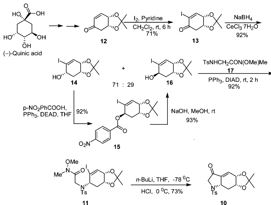
SCHEME 2. Synthesis of Chiral Azabicyclic Enone 10
