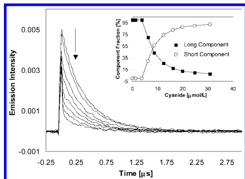
Figure 3. Changes in the time-resolved PL decay of sensor 1 ( 9.04\ \mu\text{M} ) upon the addition of cyanide ( 0\text{--}32\ \mu\text{M} ), obtained with 458\ \text{nm} excitation. (Inset) Shifts in fractional intensity of the two lifetime components obtained from biexponential analysis. See text for details.
