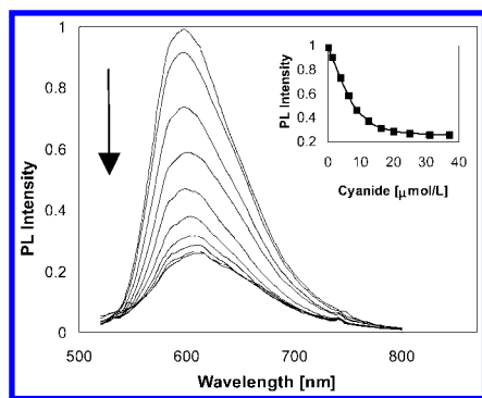
Figure 2. Changes in photoluminescence intensity of sensor 1 ( 9.04\ \mu\text{M} ) in \text{CH}_2\text{Cl}_2/\text{CH}_3\text{CN} (98:2) upon the addition of cyanide ( 0\text{--}38.79\ \mu\text{M} ). (Inset) Binding isotherm monitored by the integrated luminescence intensity. \lambda_{\text{ex}} = 493\ \text{nm} (isosbestic point in UV–vis spectra).
