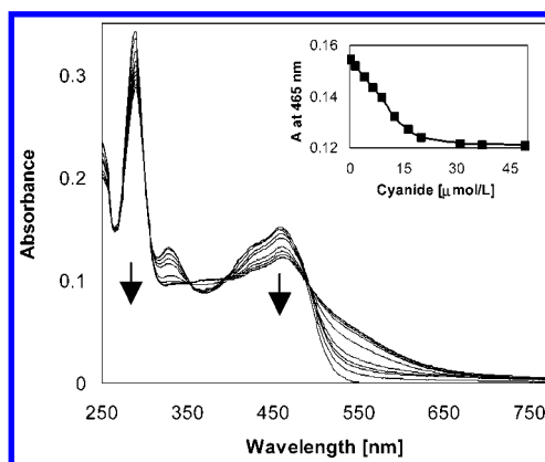
Figure 1. Changes in the UV-vis spectrum of sensor 1 (9.04 \mu M in CH 2 Cl 2 /CH 3 CN (98:2)) upon the addition of cyanide (0–49.02 \mu M). (Inset) Binding isotherm monitored by the absorbance decrease at 465 nm.
