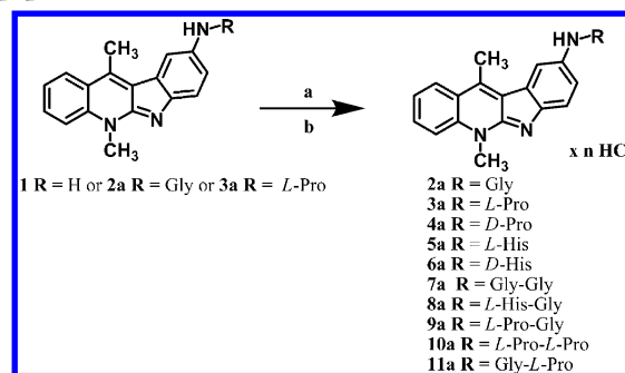
Scheme 1. Synthesis of Hydrochloride Amino Acid and Dipeptide Derivatives of DiMIQ a
