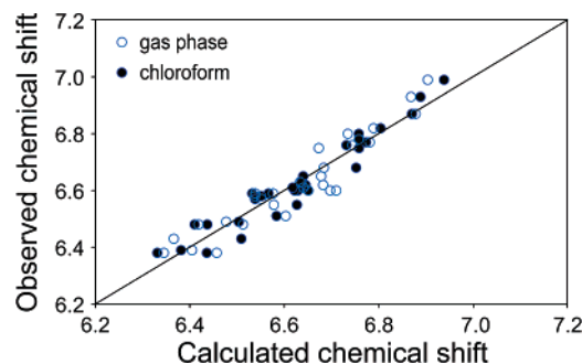
FIGURE 6. Comparison of observed and calculated chemical shifts of 3–16 . Calculated nuclear shieldings averaged for all conformations within 8 kJ/mol were converted to calculated chemical shifts by use of the regression equations for all compounds (see text).
