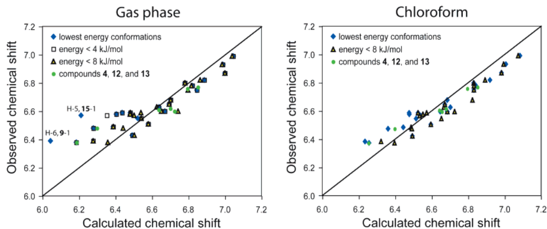
FIGURE 5. Comparison of observed and calculated chemical shifts of 3–16 . For compounds 3 , 5–11 , and 14–16 , the calculated nuclear shieldings were converted to chemical shifts by use of the regression equations derived for all chemical shifts of compounds 4 , 12 , and 13 (Figure 4). Calculated chemical shifts for the minimum-energy conformations, averaged chemical shifts for all conformations with calculated energies within 4 kJ/mol, and averaged chemical shifts for all conformations with calculated energies within 8 kJ/mol are displayed separately.
