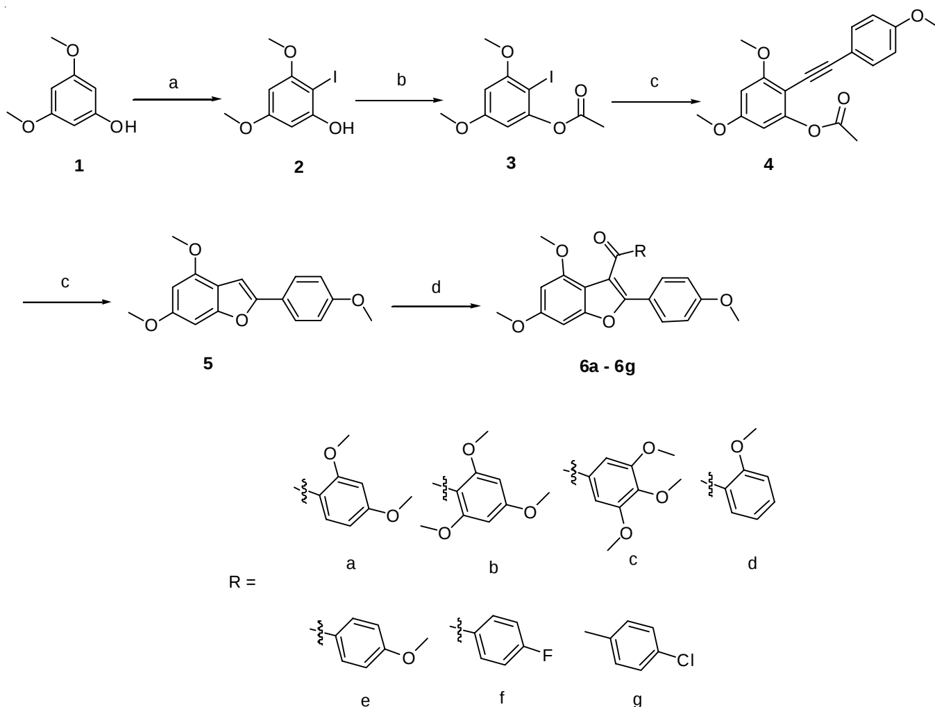
Scheme-1: Synthesis of benzo[b]furan derivatives 6a-6g
