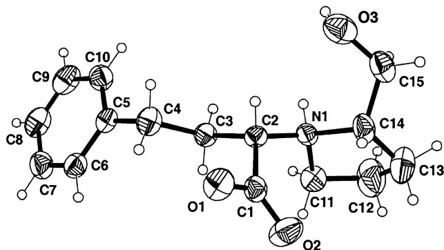
Figure 1. ORTEP view of the molecular structure of VIc (50% probability thermal ellipsoids).
