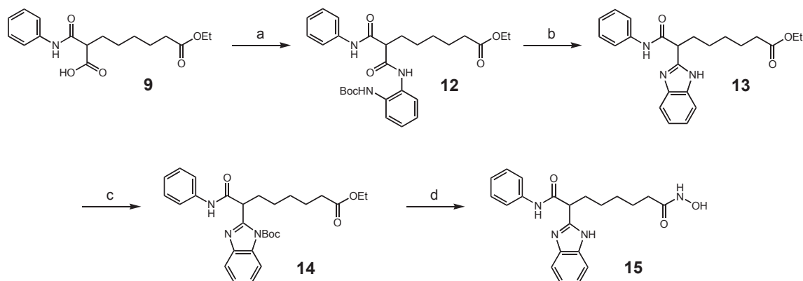
Scheme 3. Synthesis of a branched 2-benzimidazolyl derivative of SAHA. Reagents and conditions: a tert -Butyl N -(2-aminophenyl)carbamate (1 equiv.), EDC.HCl (1.1 equiv.), HOBT (1.1 equiv.), Et 3 N (2.2 equiv.), DMF, 20 °C, 18 h, 66%; b TFA, reflux, 2 h, 75%; c Di- tert -butyl dicarbonate (1.5 equiv.), THF, 20 °C, 7 d, 64% conversion; d Aqueous 50% HONH 2 (10 equiv.), 1 M KOH in MeOH, THF, 20 °C, 6 h, 50%.
