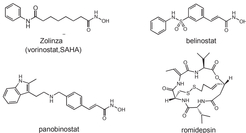
Fig. 1. FDA-approved HDAC inhibitors.
