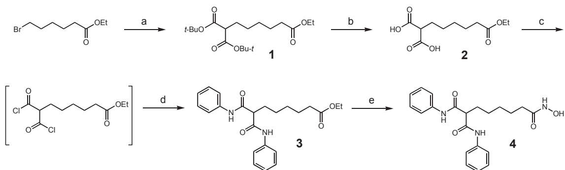
Scheme 1. Synthesis of a symmetrical bis-malonamide hydroxamic acid. 14 Reagents and conditions: a NaH (1.1 equiv.) first added to di- tert -butyl malonate (1 equiv.), THF, 20 °C, 20 min then reflux, 16 h, 74%. b CF 3 CO 2 H (6 equiv.), CH 2 Cl 2 , 20 °C, 16 h, 99%. c SOCl 2 (6 equiv.), benzene, reflux, 2 h 14 then, d PhNH 2 (6 equiv.), pyridine (3 equiv.), CH 2 Cl 2 , 20 °C, 17 h, 76%. e NaOMe, (3 equiv.) and HONH 2 (2 equiv.), MeOH, 20 °C, 16 h, 68%. 14
