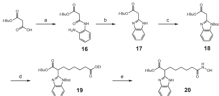
Scheme 4. Synthesis of a branched hydroxamic acid with a 2-benzimidazolyl capping group. Reagents and conditions: a 1,2-Phenylenediamine (1 equiv.), N,N' -dicyclohexylcarbodiimide (1.1 equiv.), MeCN, 20 °C, 20 min, 50%. b AcOH, 90 °C, 1 h, 96%. c Di- tert -butyl dicarbonate (1.2 equiv.), THF, 20 °C, 3 d, 97%. d NaH (1.1 equiv.), THF, 60 °C, 18 h, 33%. e 50% aqueous HONH 2 (10 equiv.), 1 M KOH in MeOH, THF, 20 °C, 30 min, 67%.
