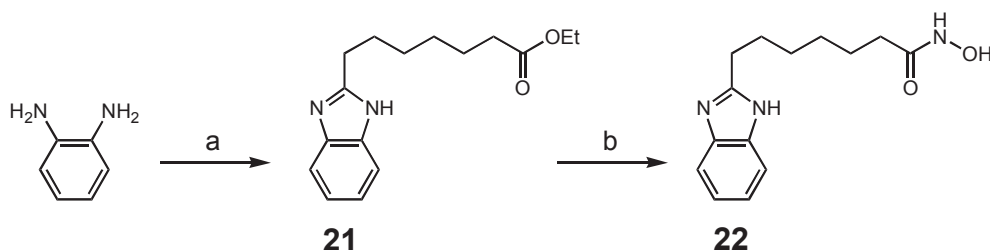
Scheme 5. Succinct synthesis of a linear hydroxamic acid with a 2-benzimidazolyl capping group. Reagents and conditions: a Suberic anhydride (1 equiv.), THF, 20 °C, 20 min; then 4% conc. H 2 SO 4 in EtOH, 29%. b Aqueous 50% HONH 2 , 1 M KOH in MeOH, THF, 20 °C, 6 h, 61%.
