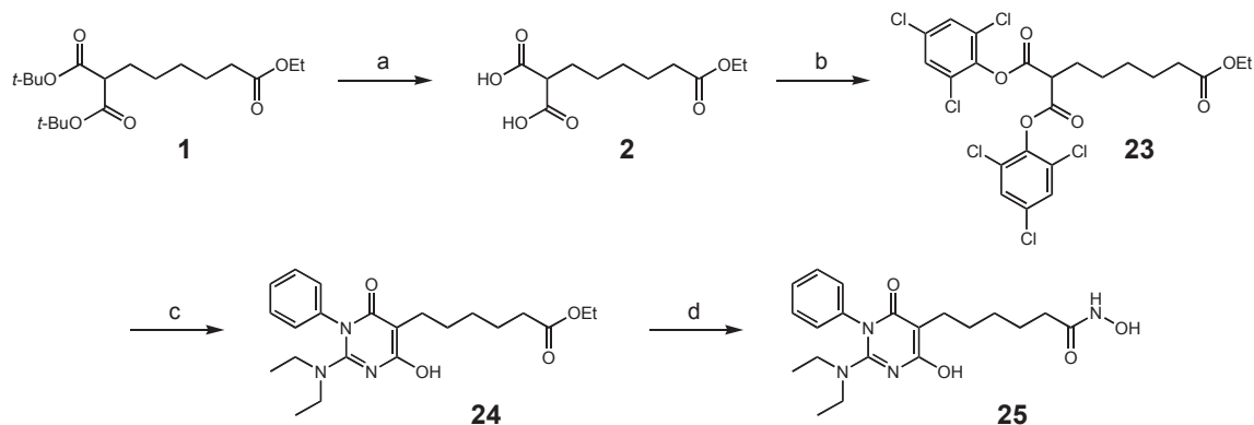
Scheme 6. Synthesis of a SAHA analog constrained by annulation. Reagents and conditions: a CF 3 CO 2 H (6 equiv.), CH 2 Cl 2 , 20 °C, 24 h, 99%. b 2,4,6-Trichlorophenol (2 equiv.), POCl 3 (2.6 equiv.), 100 °C, 5 h, 49%. c N,N -Diethyl- N' -phenylguanidine (1 equiv.), 5 min, 150 °C, 68%. d Aqueous 50% HONH 2 (10 equiv.), 1 M KOH in MeOH, THF, 20 °C, 2 h, 51%.
