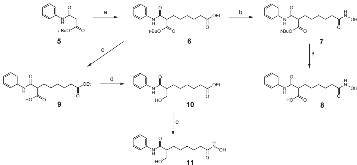
Scheme 2. Synthesis of branched derivatives of SAHA. Reagents and conditions: a NaH (1.1 equiv.), ethyl 6-bromohexanoate (1 equiv.), THF, 70 °C, 18 h, 74%; b 50% aqueous HONH 2 (10 equiv.), 1 M KOH in MeOH, THF, 20 °C, 1 h, 29%; c 1:1 CF 3 CO 2 H:CH 2 Cl 2 , 20 °C, 6 h, 80%; d ClCO 2 Et (1.5 equiv.), Et 3 N (1.2 equiv.), THF, 0 °C, 30 min then NaBH 4 (3 equiv.), 21 MeOH, 10 °C, 1.5 h, 77%; e Aqueous 50% HONH 2 (5 equiv.), 1 M KOH in MeOH, THF, 20 °C, 1.5 h, 12%; f 1:1 CF 3 CO 2 H:CH 2 Cl 2 , 20 °C, 30 min, 80%.
