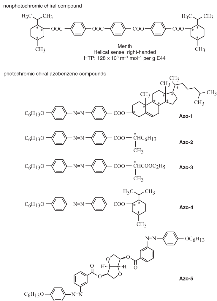
Figure 1. Structures of photochromic and nonphotochromic chiral compounds used in this study.
