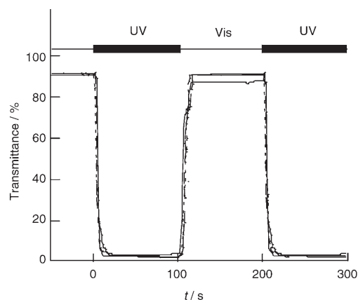
Figure 9. Changes in diode laser (670 nm) transmittance through (E44/Chiral/Azo-5) mixtures in a homogeneous glass cell on UV ( 3.2 \text{ mW cm}^{-2} ) and visible light ( 8.3 \text{ mW cm}^{-2} ) irradiation at 25^\circ\text{C} . Compositions of (E44/Chiral/Azo-5) mixtures are: 80:9.8:10.2 wt % (—), 75:12.3:12.7 wt % (----), and 70:14.8:15.2 wt % (- - -).
